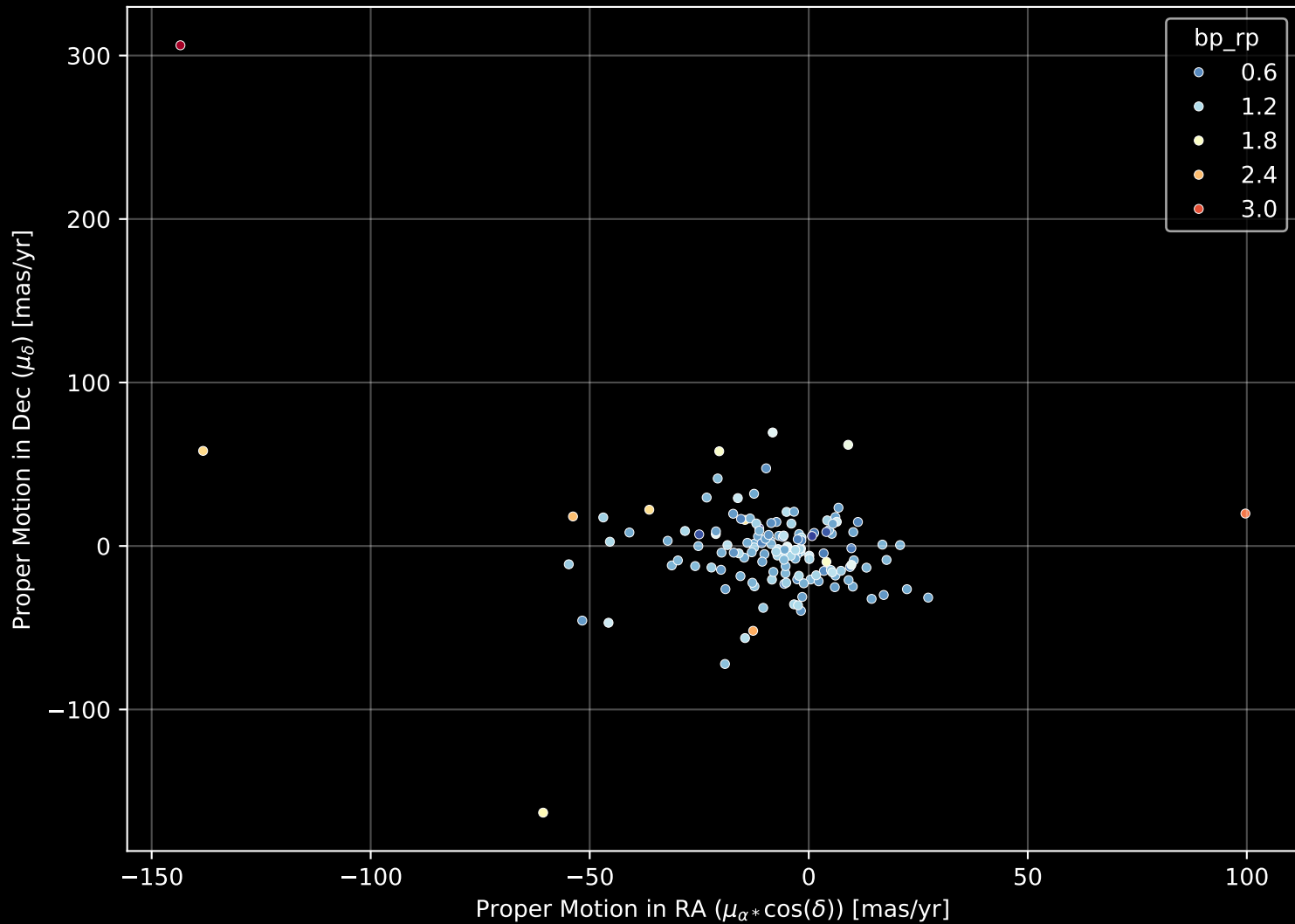
APOGEE DR17 Field: [064+42_MGA] Proper Motion Diagram (n= 147)
