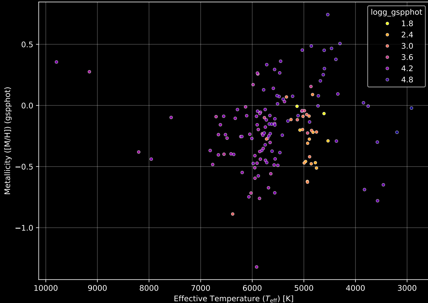
APOGEE DR17 Field: [064+42_MGA] Stellar Population Parameters (n= 147)
