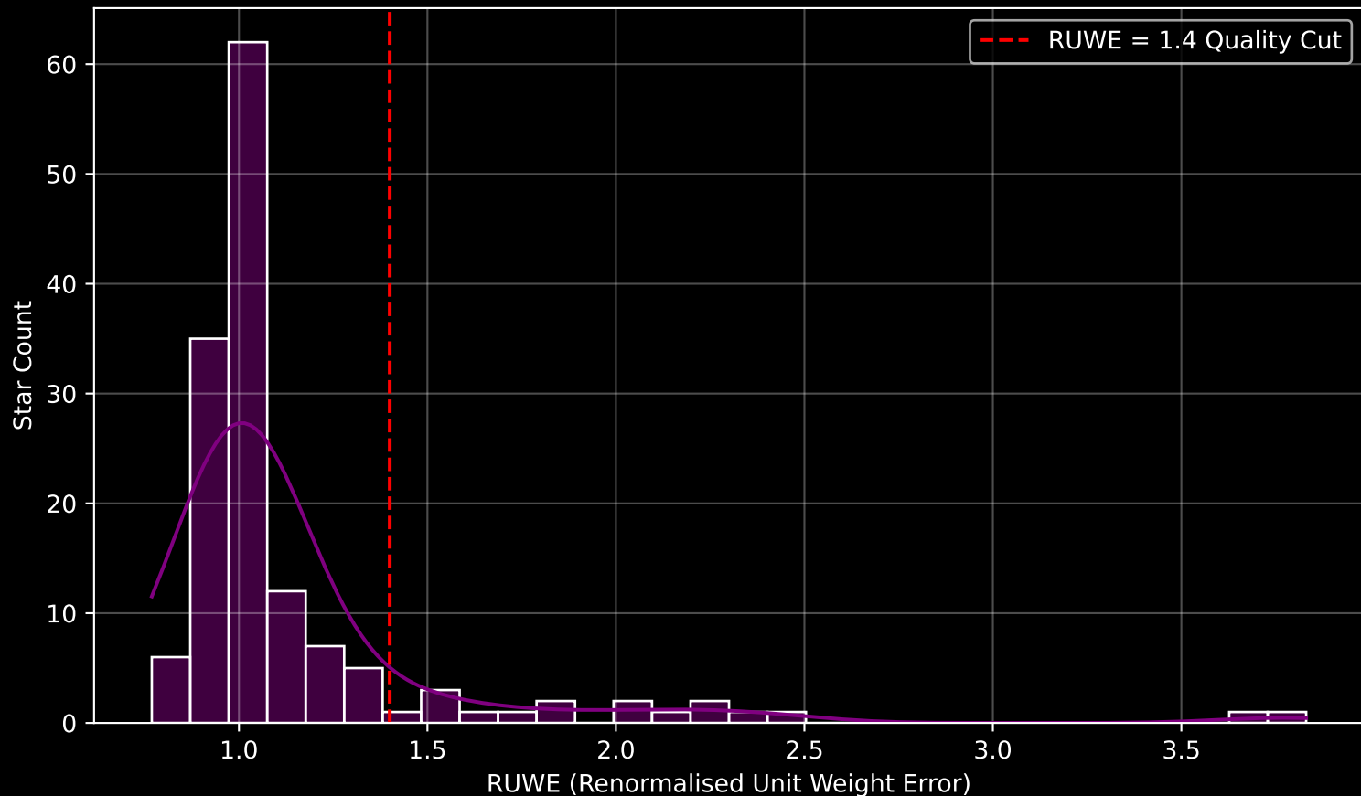
GAPOGEE DR17 Field [064+42_MGA] RUWE Distribution (n= 144)
