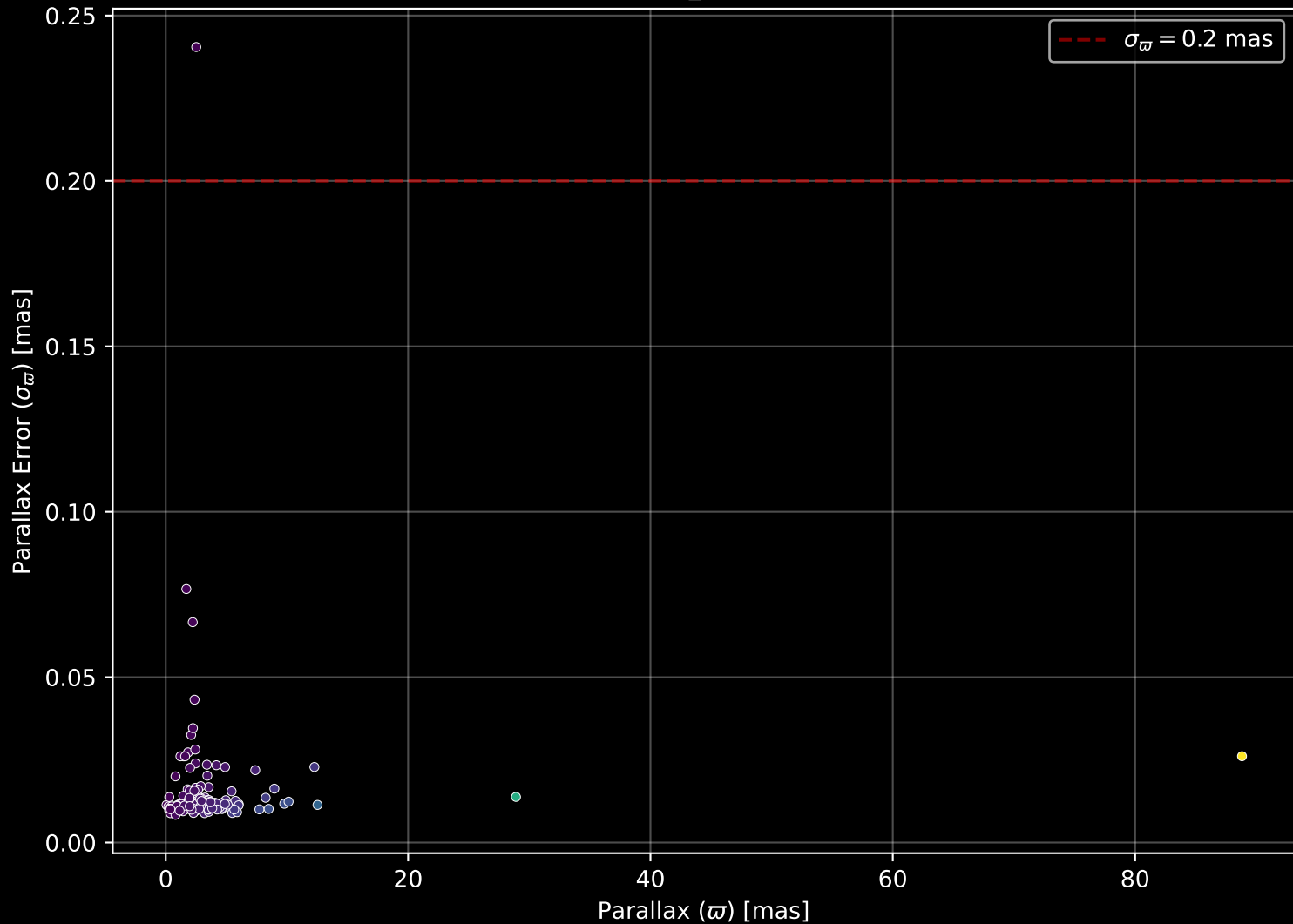
APOGEE DR17 Field: [064+42_MGA] Parallax Quality (n= 147)
