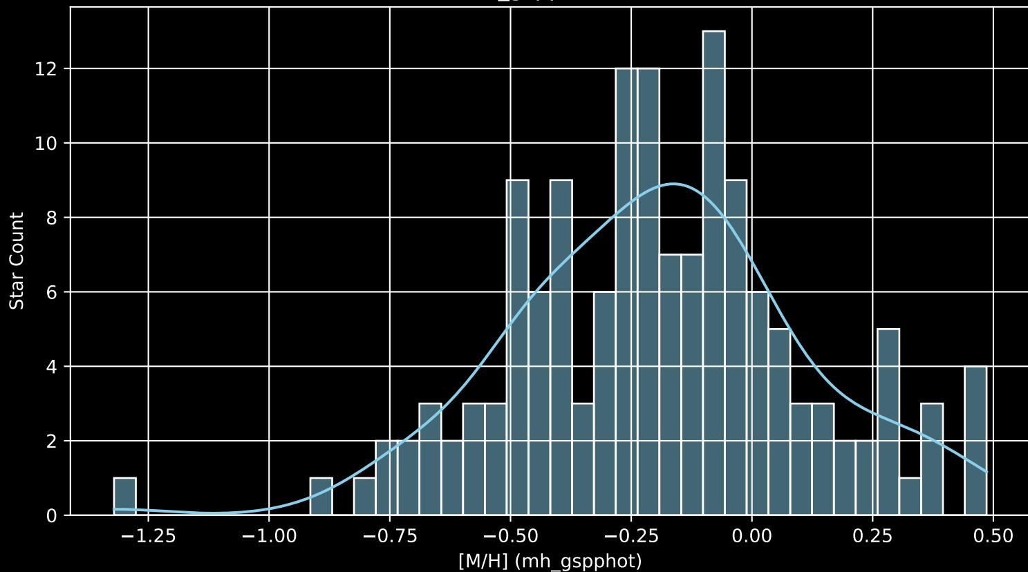
APOGEE DR17 Field: [064+42_MGA [M/H] (mh_gspphot) (n= 145)
