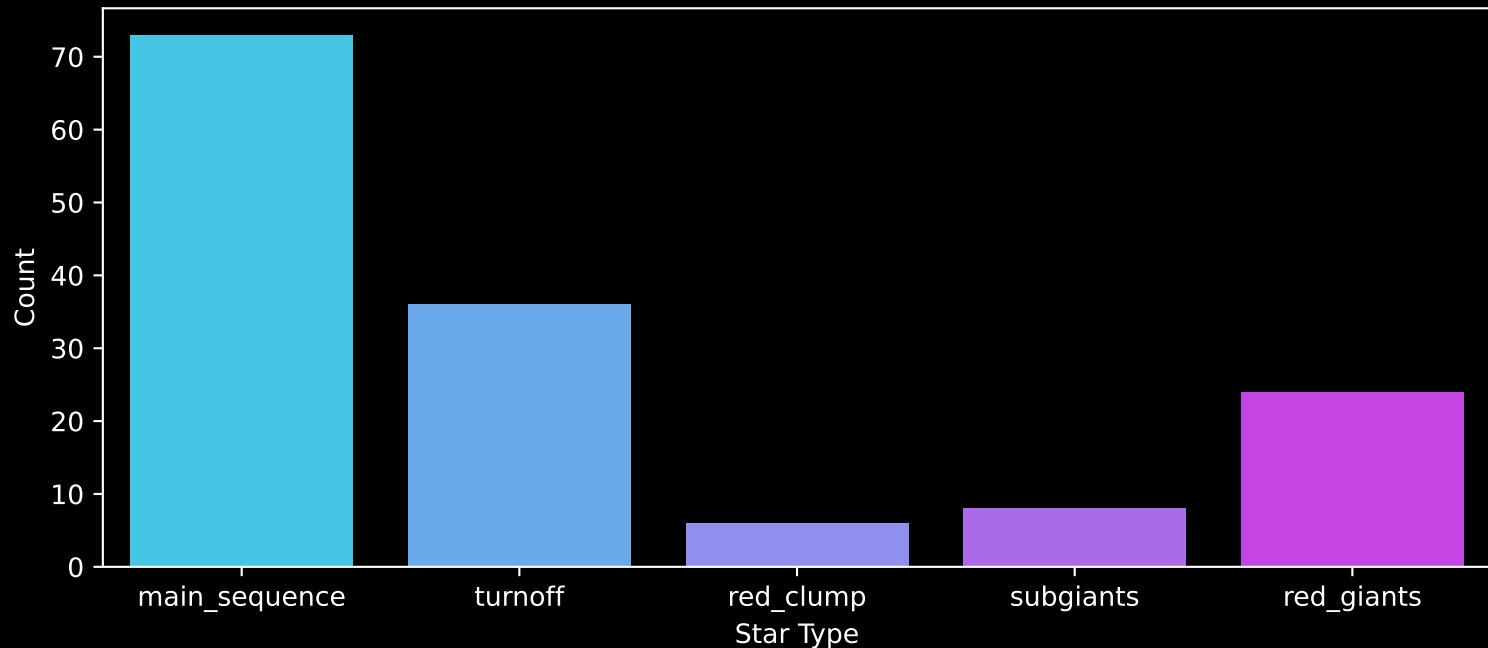
APOGEE DR17 Field: [064+42_MGA] Count plot of Star Type
