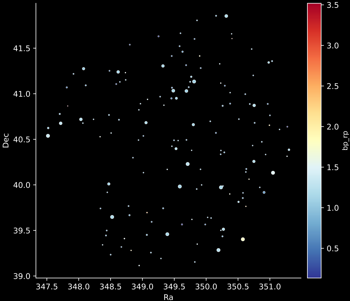
APOGEE DR17 Field: [064+42_MGA] Stars: 147
